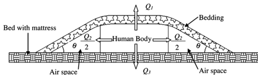
Fig. 2. Schematic of heat transfer pathways in a bedding system including a sleeping occupant (from [22]).
